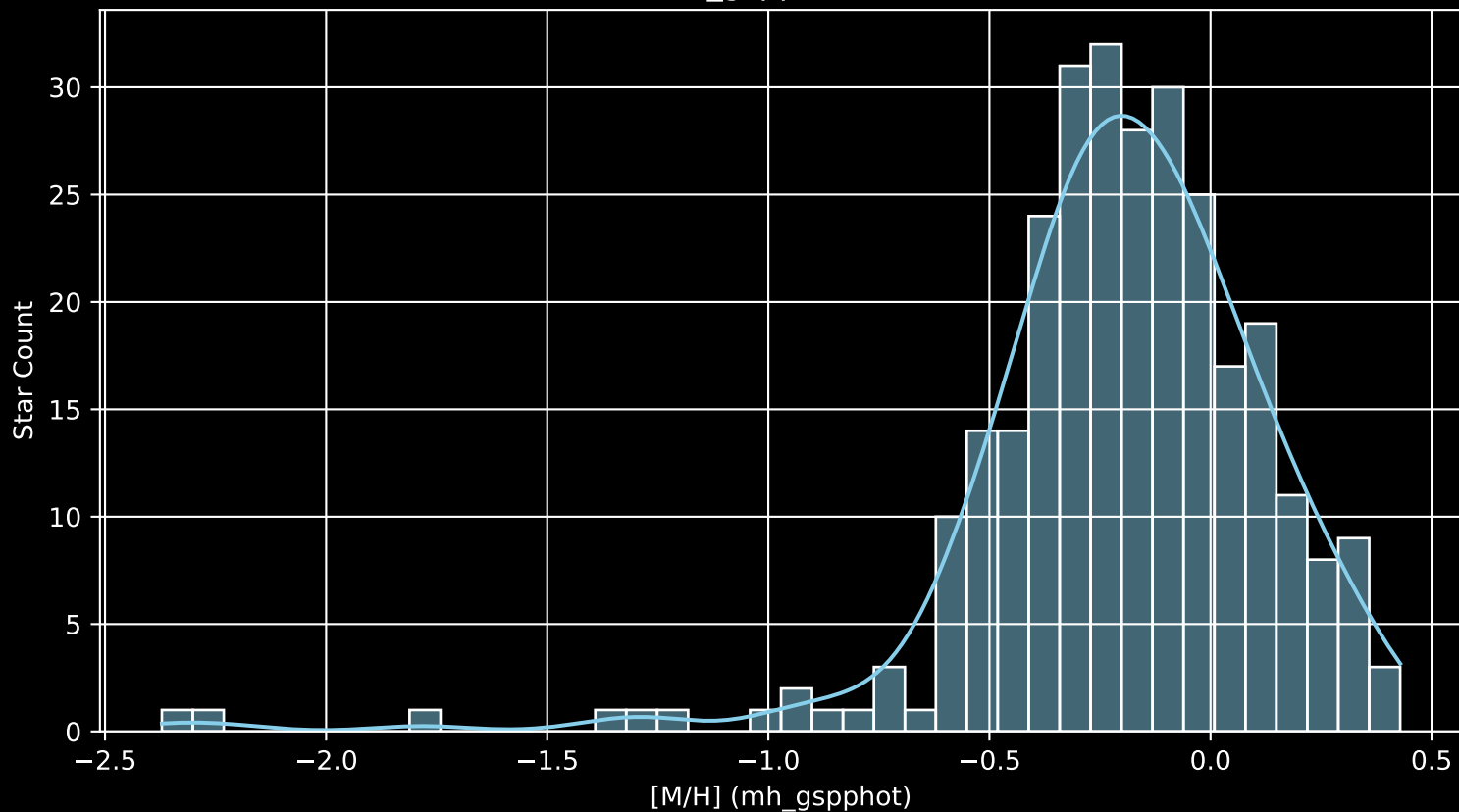
APOGEE DR17 Field: [057+35_MGA [M/H] (mh_gspphot) (n= 290)
