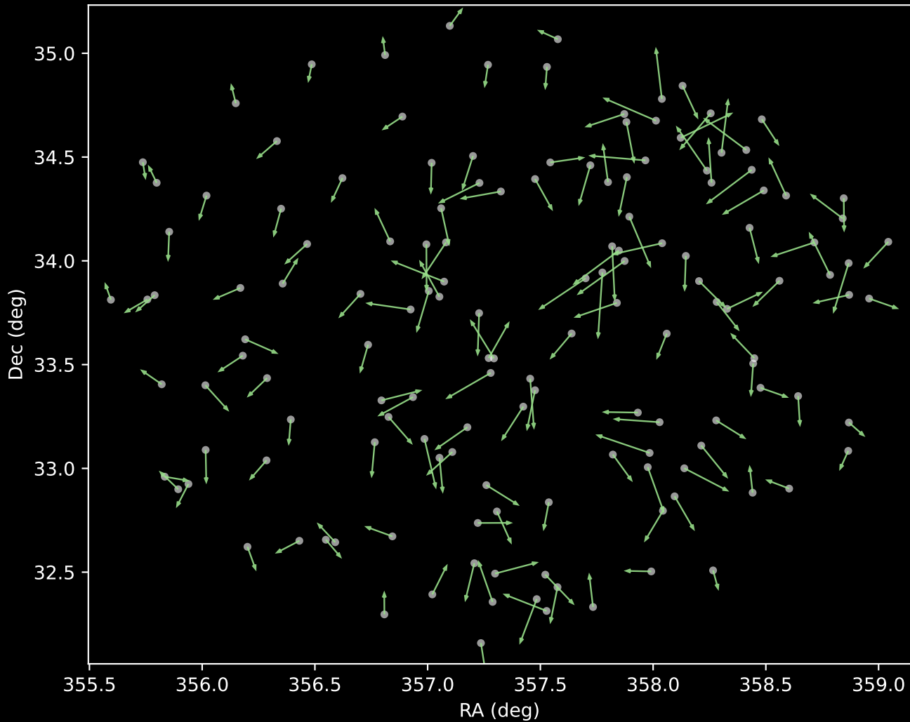
APOGEE DR17 Cluster 5 Proper Motion Vectors (n=146)
