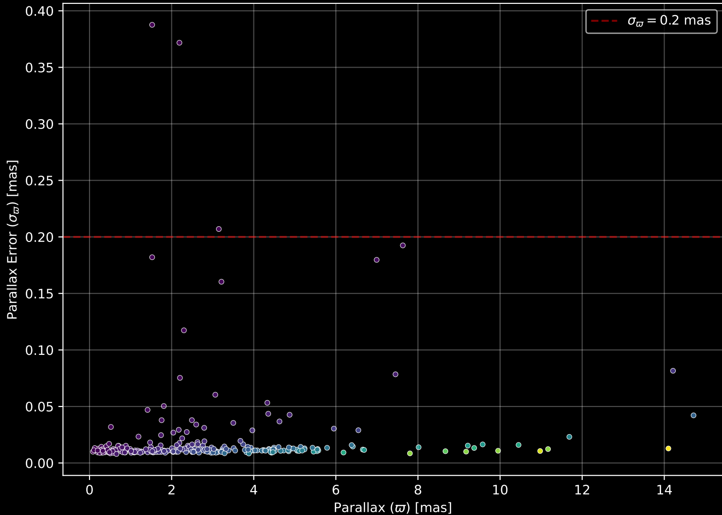
APOGEE DR17 Field: [057+35_MGA] Parallax Quality (n= 294)
