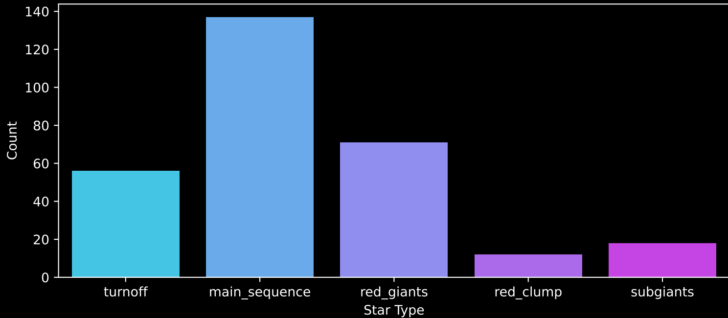
APOGEE DR17 Field: [057+35_MGA] Count plot of Star Type
