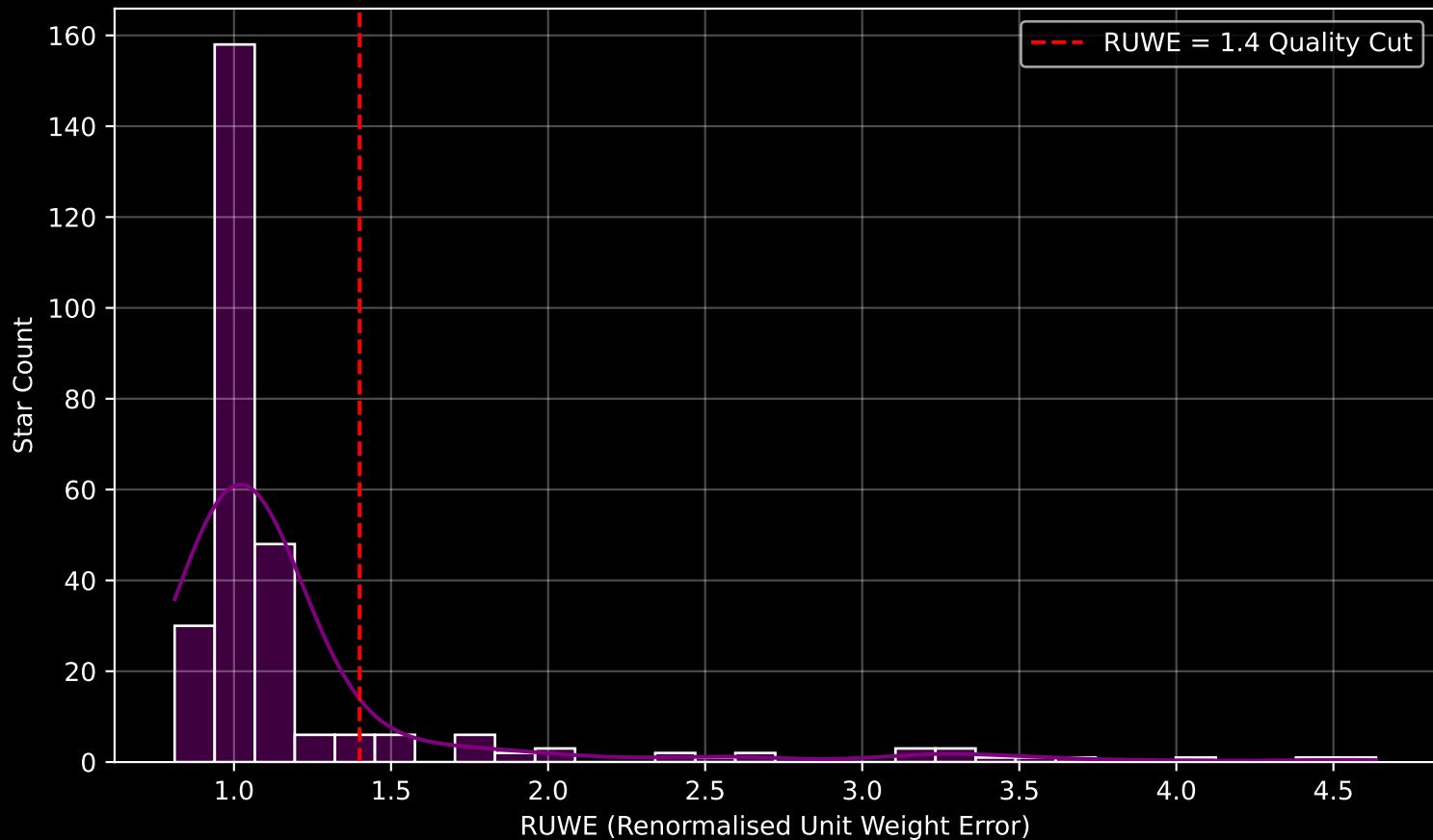
GAPOGEE DR17 Field [057+35_MGA] RUWE Distribution (n= 282)
