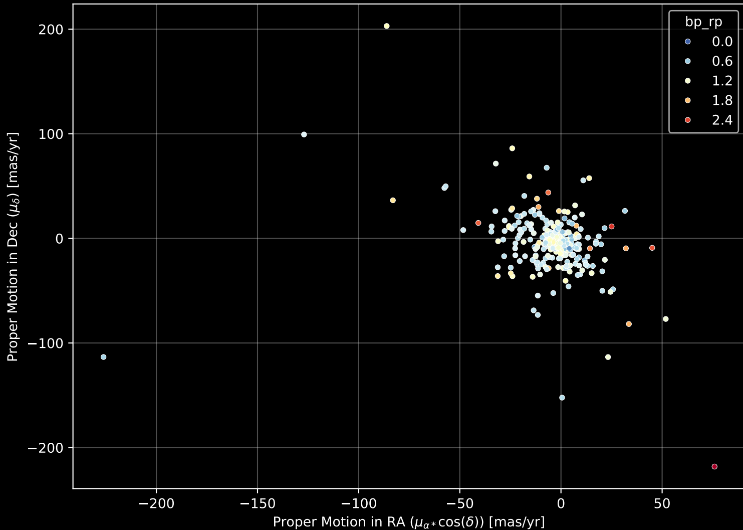
APOGEE DR17 Field: [057+35_MGA] Proper Motion Diagram (n= 294)
