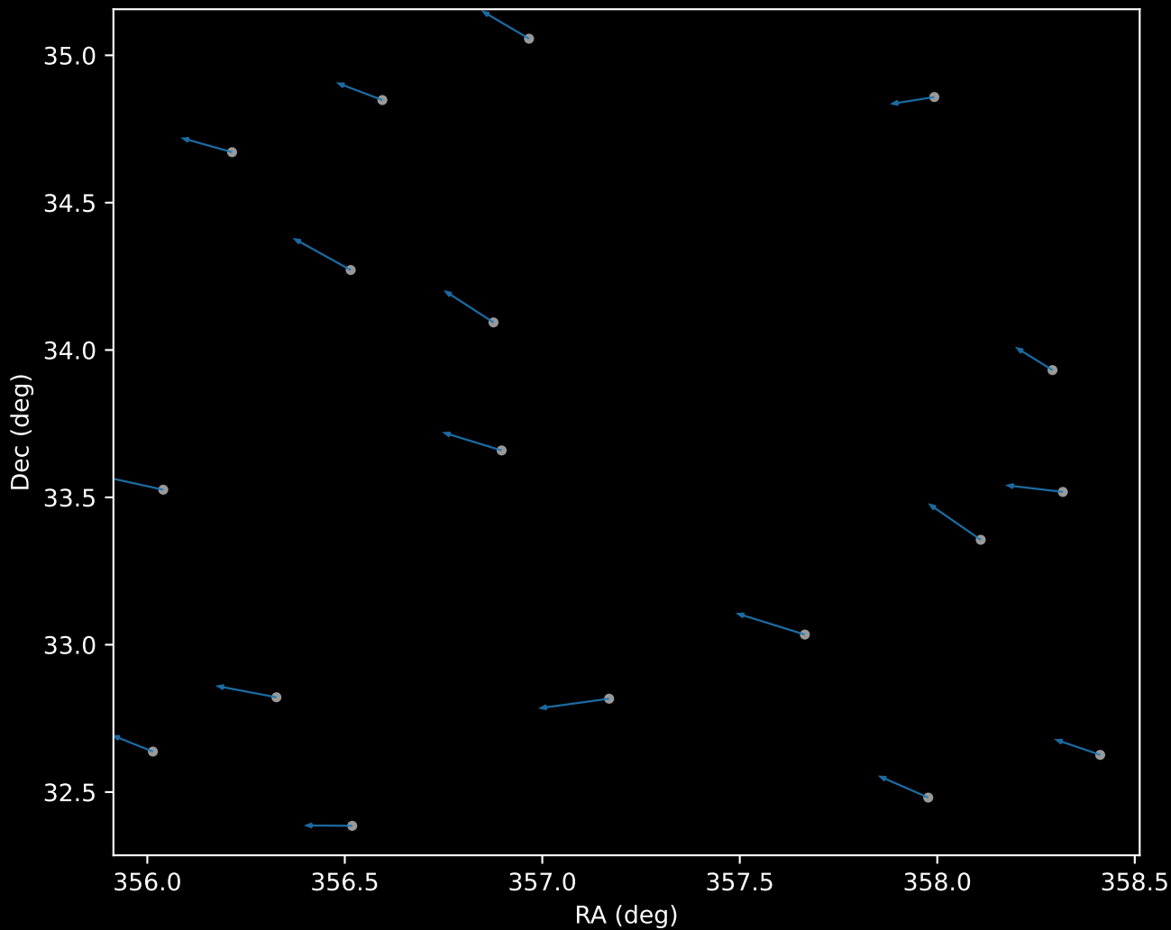
APOGEE DR17 Cluster 0 Proper Motion Vectors (n=18)
